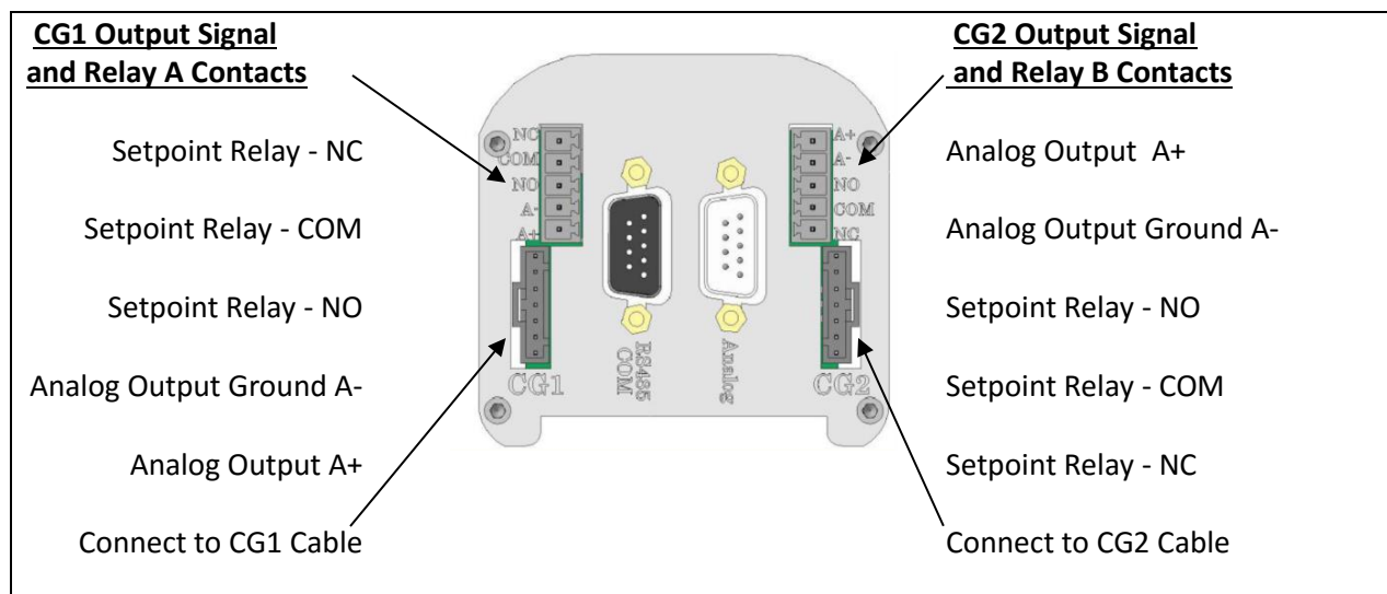
IGM402 I/O Terminal Blocks for CG1, CG2, RELAY A and RELAY B
